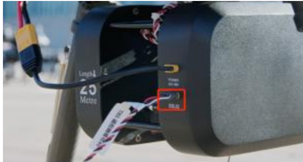
FIG 5-4-2 The SBUS cable into the winch SBUS
